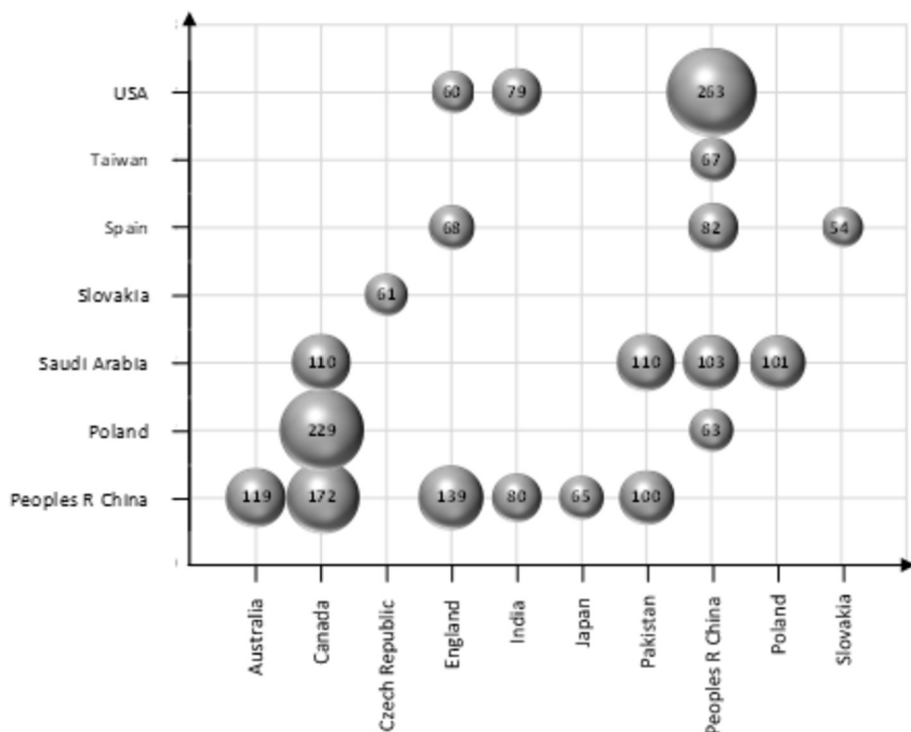
Fig. 9. The co-occurrence of countries with link strength in the interval (50; 263].
