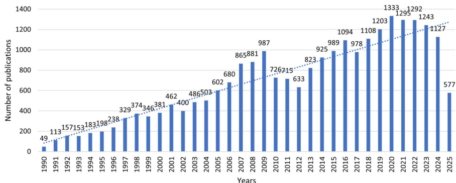
Fig. 2. Chronological distribution of the published papers on fuzzy sets (RQ1).
