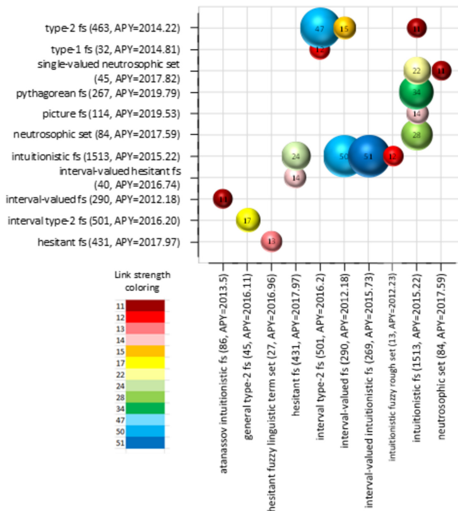
Fig. 7. The co-occurrence matrix of fuzzy set extensions with link strengths (10; 51].
