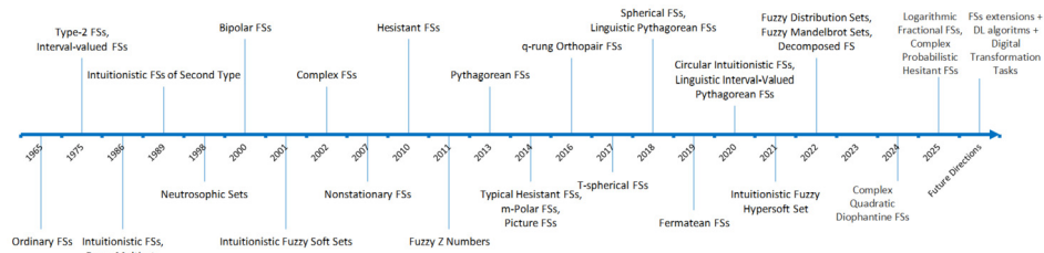
Fig. 12. Evolution of fuzzy sets.
