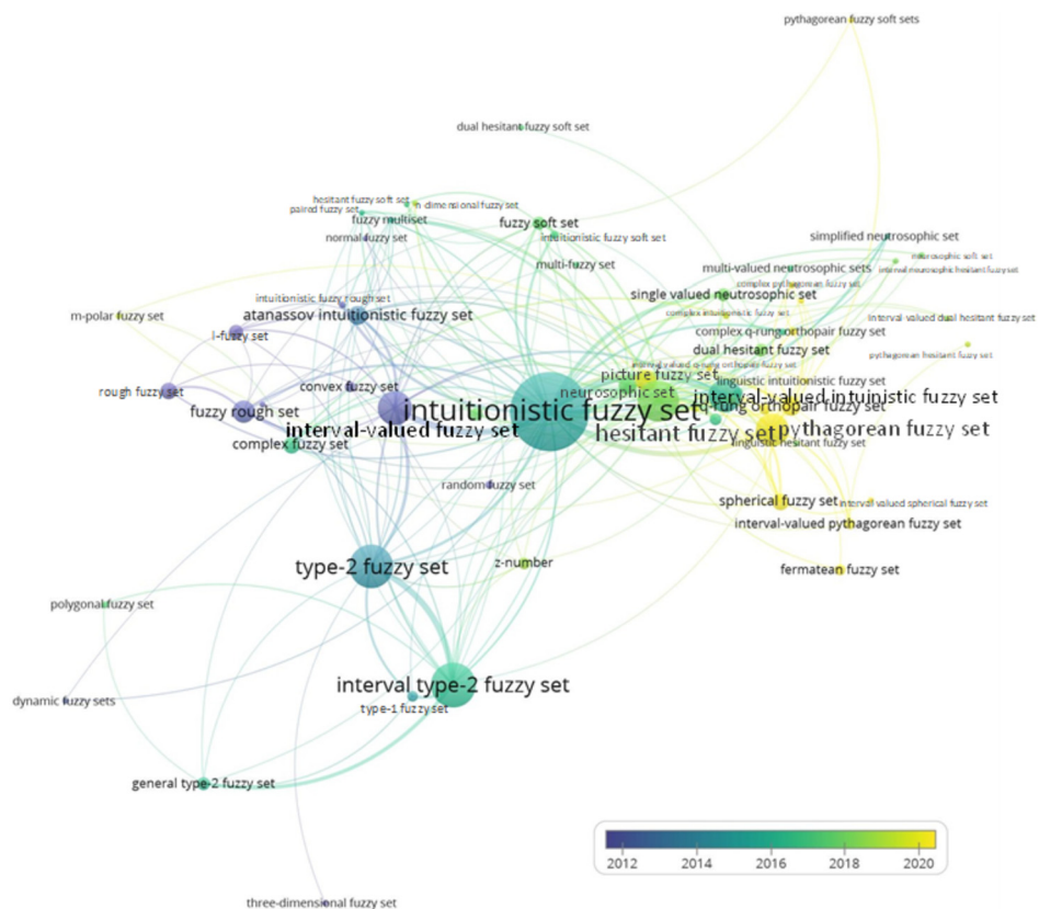
Fig. 4. Keyword map on fuzzy set extensions according to years (RQ2).
