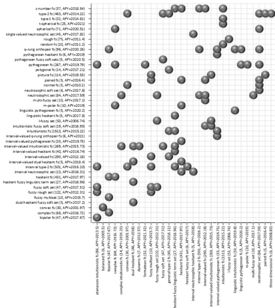
Fig. 5. The co-occurrence matrix of fuzzy set (fs) extensions with link strengths 1.
