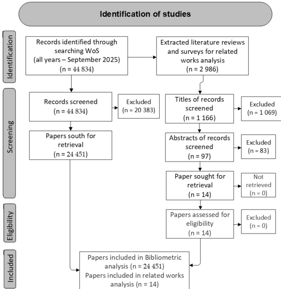
Fig. 1. The schema of the current bibliometric analysis (adopted from Yepes-Núñez et al. , 2021).
