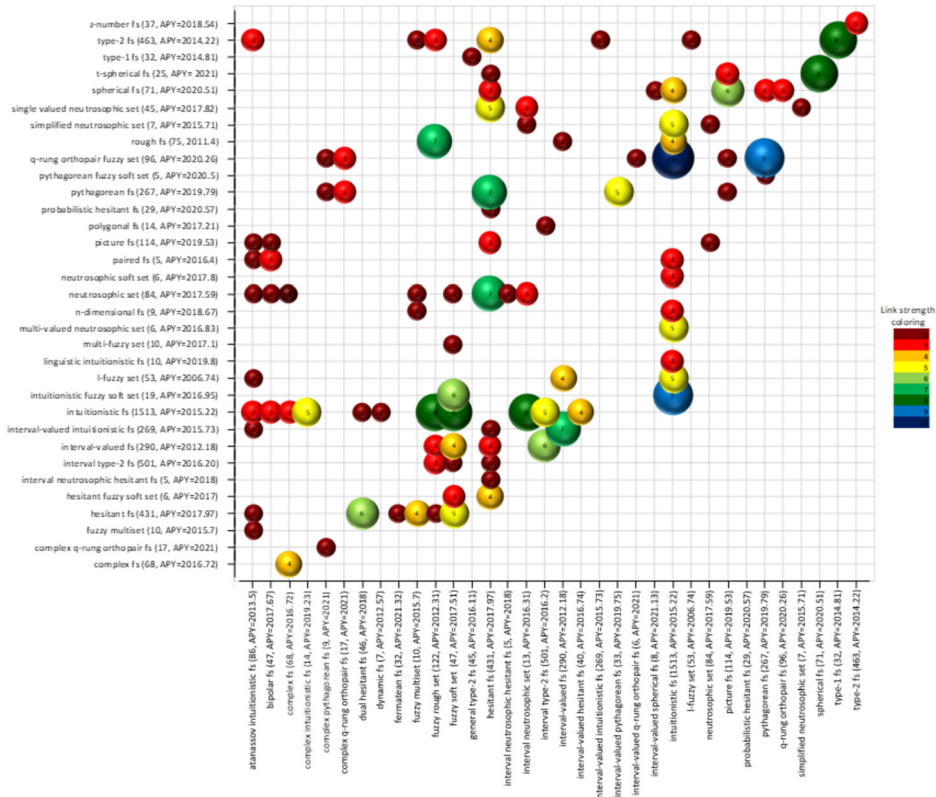
Fig. 6. The co-occurrence matrix of fuzzy set extensions with link strengths (1; 10].
