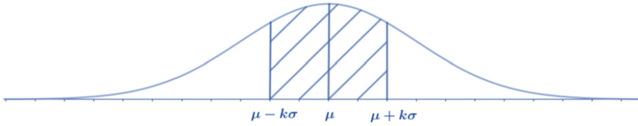
Fig. 6. Chebyshev's inequality.
